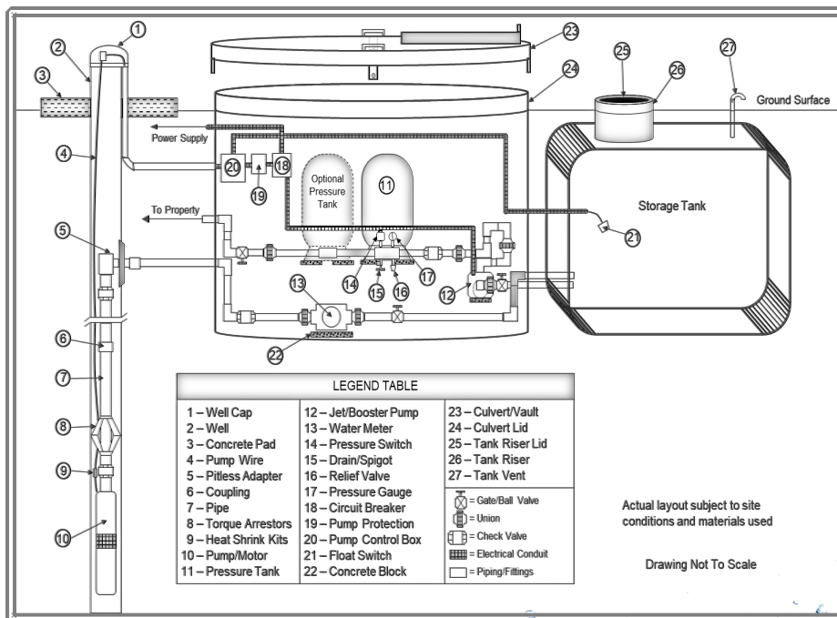
Typical System layout. System Layouts vary from sit to site.
